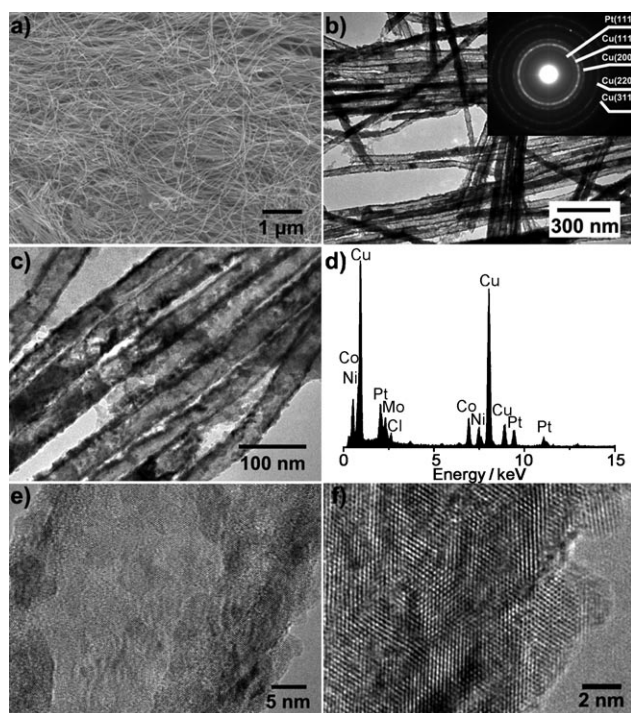
Figure 1. Structural characterization of the \text{Pt}_5\text{Cu}_{76}\text{Co}_{11}\text{Ni}_8 nanotubes. a) A representative SEM micrograph of the nanotubes released from AAO membranes. b, c) Typical TEM micrographs. Inset of (b): Electron diffraction pattern. d) EDX spectrum. e, f) High-resolution TEM images.
